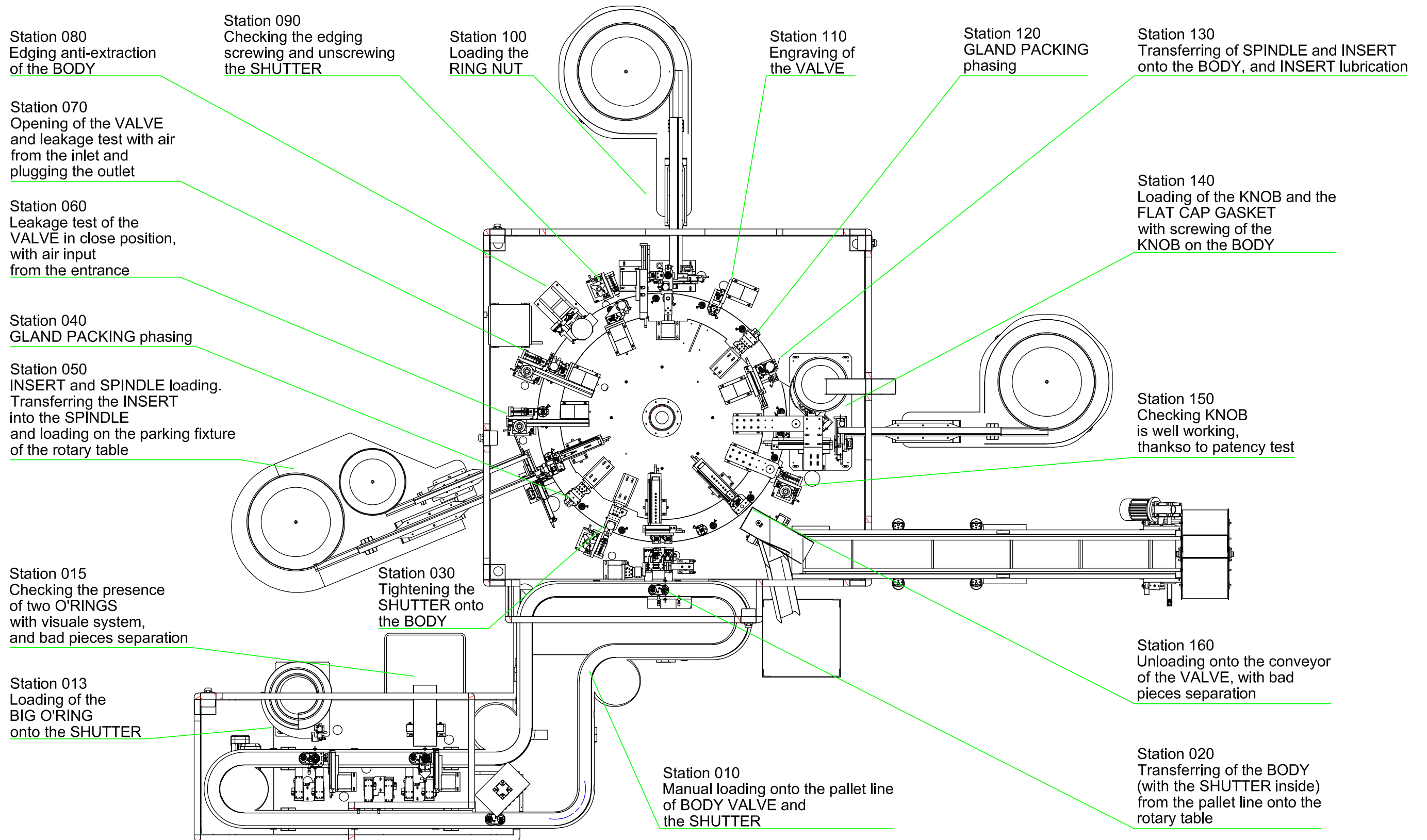
AUTOMATIC MACHINE FOR ASSEMBLING AND TESTING RADIATOR VALVES
