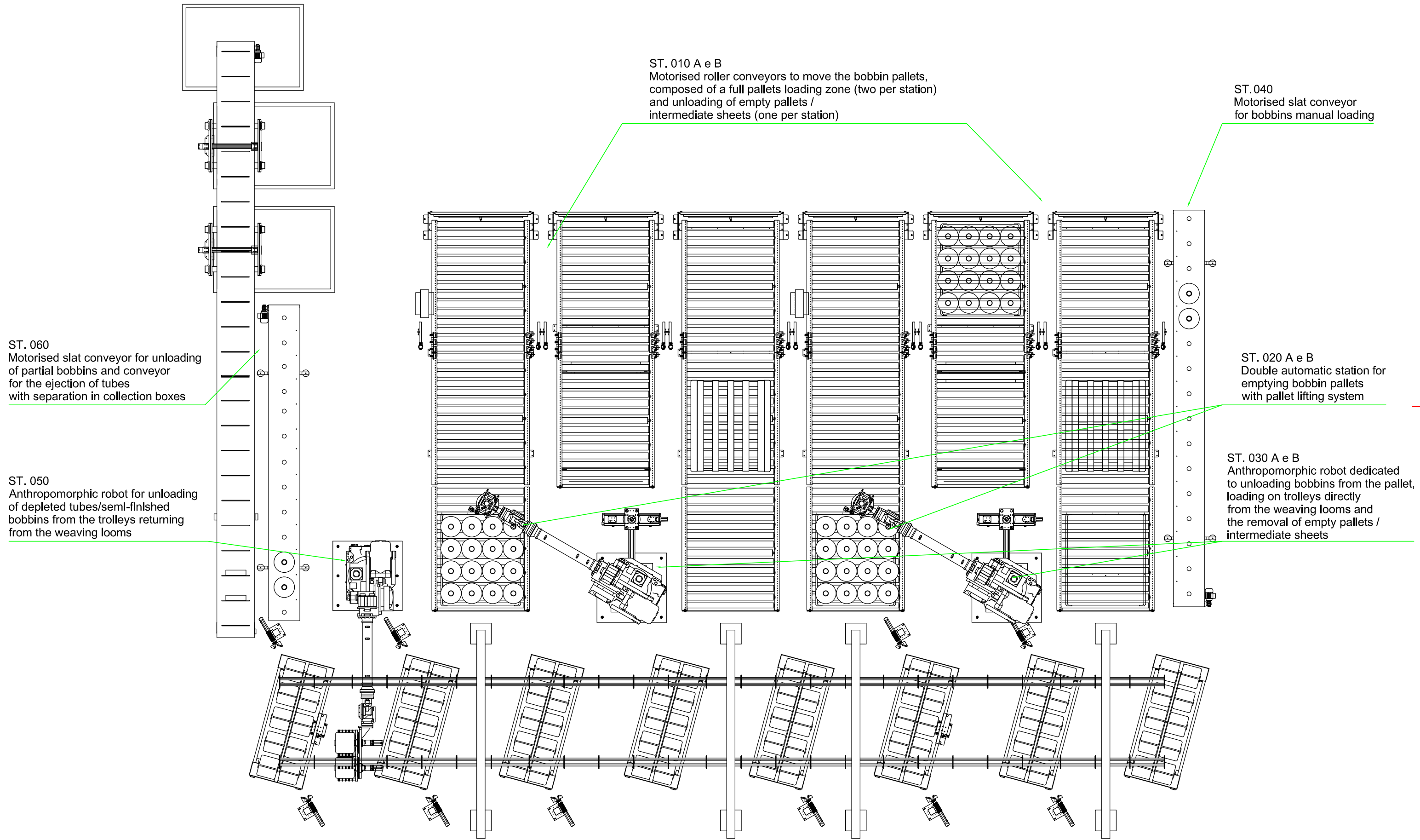
AUTOMATIC CREELING SYSTEM FOR TUFTING MACHINES (bobbins loading and tubes unloading)
